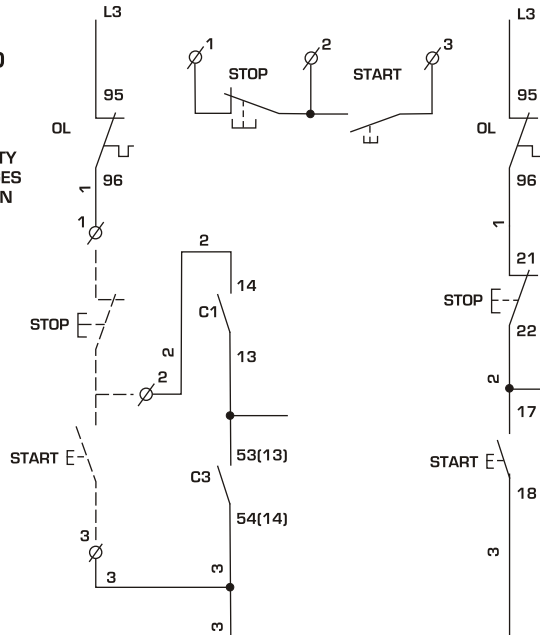
MODIFICATION FOR REMOTE CONTROL
